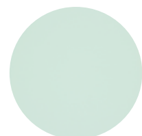
Sea Ice
